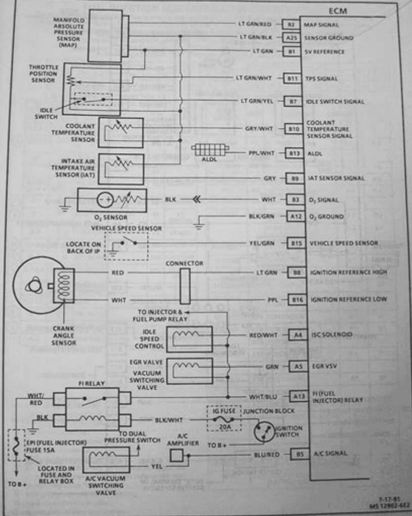
Figure A-2 - ECM Wiring Diagram (1 of 2)
